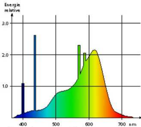
Spectre combiné
