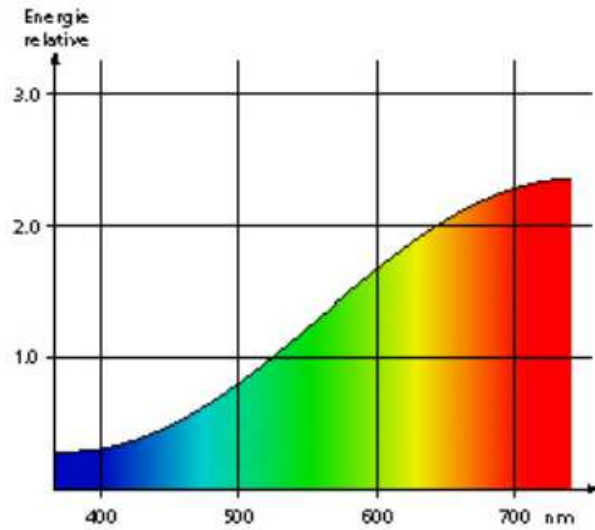
Spectre continu
