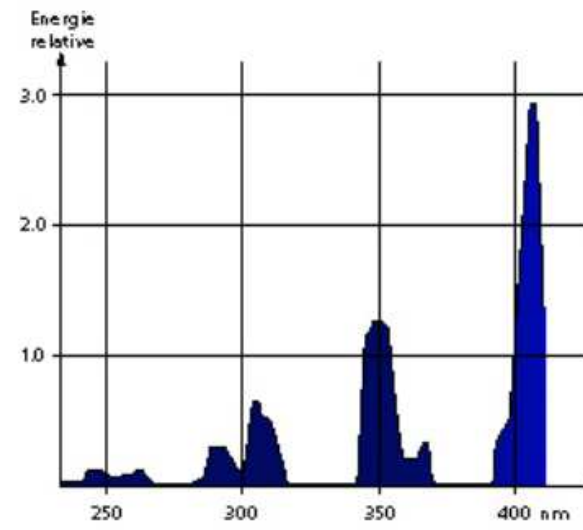
Spectre discontinu
